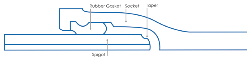
Structure of DI Pipe (push-on joint)
