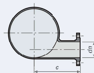
INVERT SCOUR TEE
